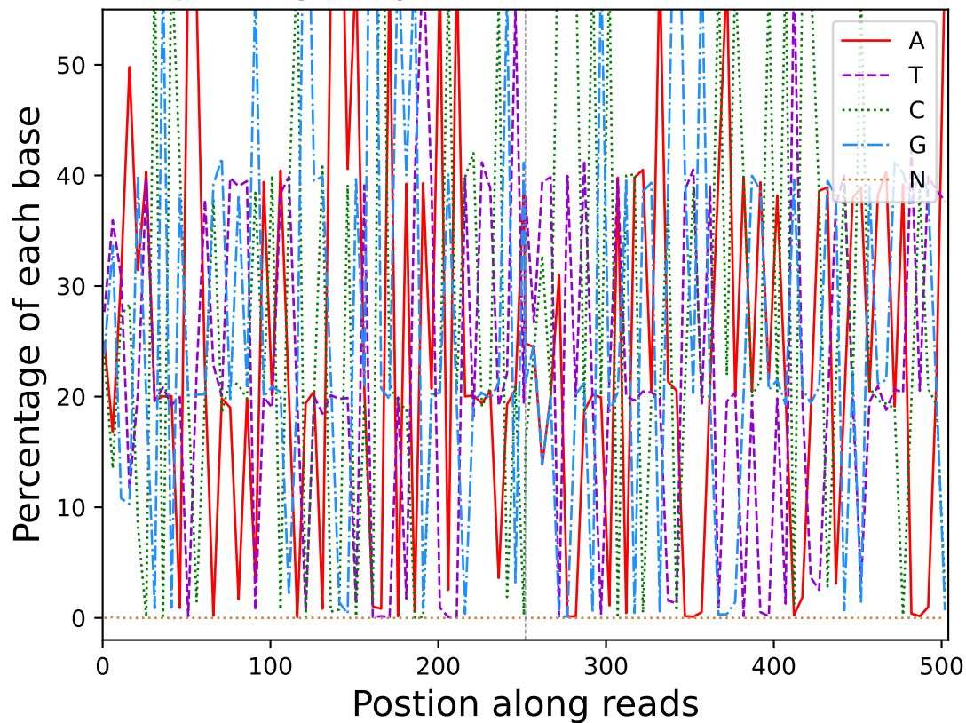
Base percentage along reads (R10926)
